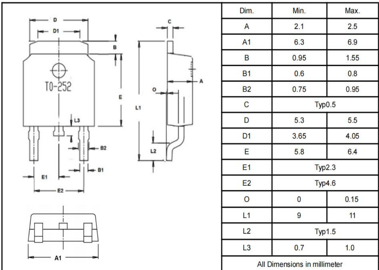
T0-252
