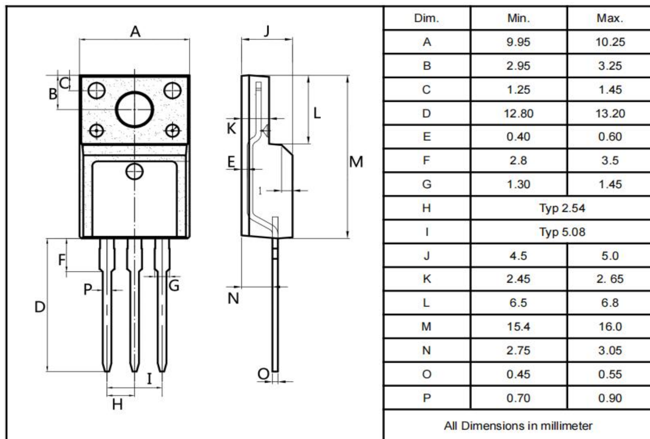
TO-220F
