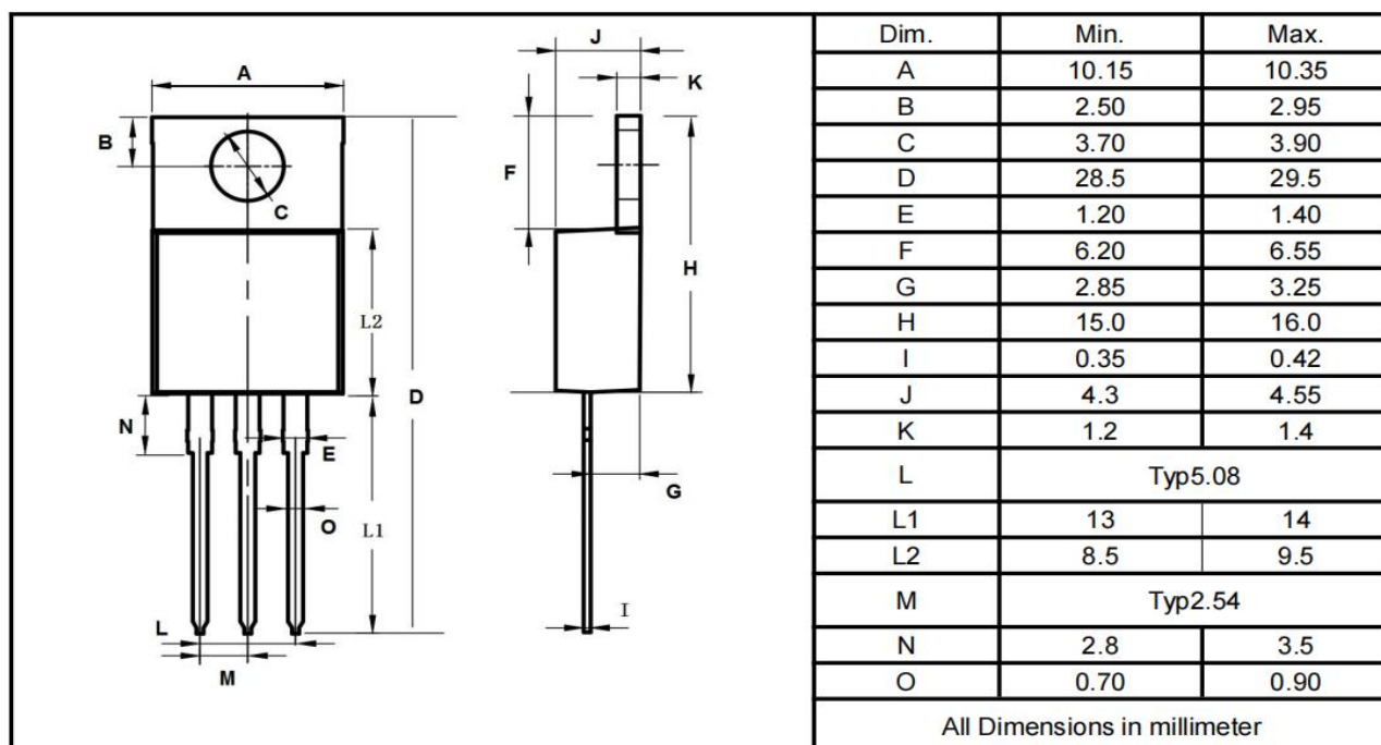
TO-220F
